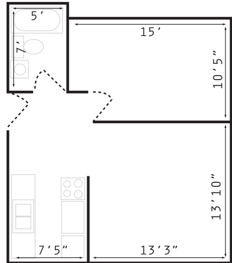
1 BEDROOM | DOUBLE APARTMENTS 203, 303
