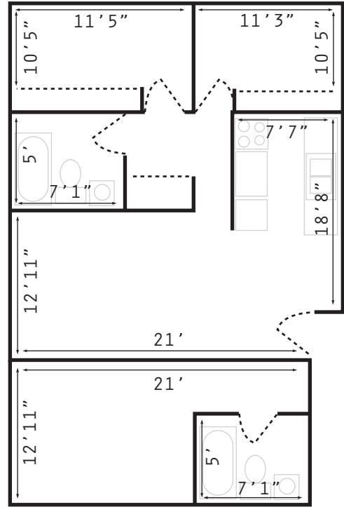
3 BEDROOM QUAD APARTMENT 102
