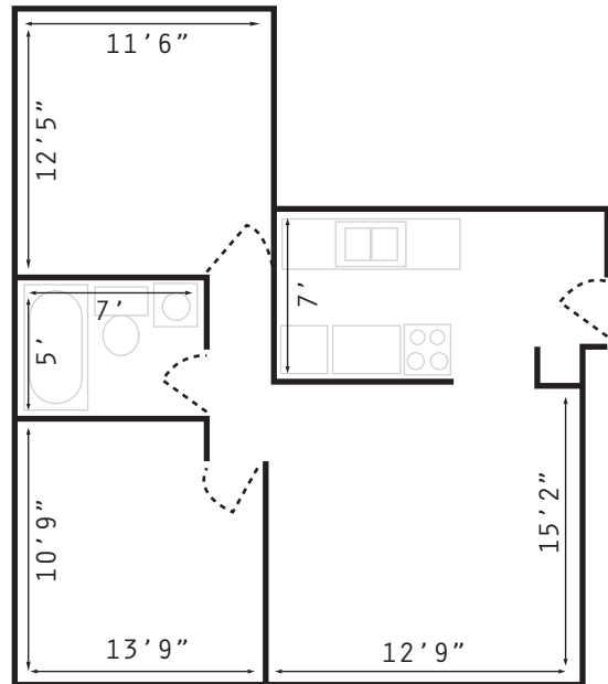
2 BEDROOM | QUAD APARTMENTS 107, 207, 307
